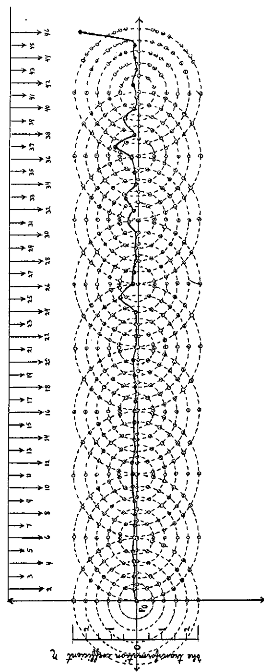
FIGURE 1. Transformation of the points of FIGURE I and SCHEME I
