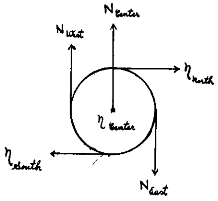
Relatively flat surface.
