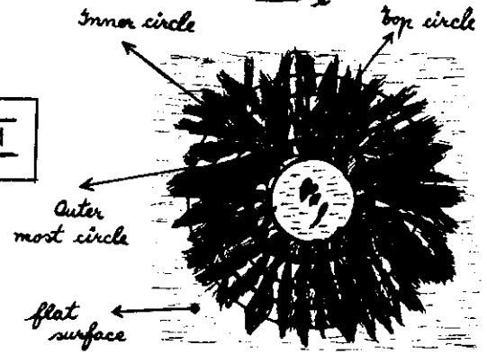
Extended rims crater
