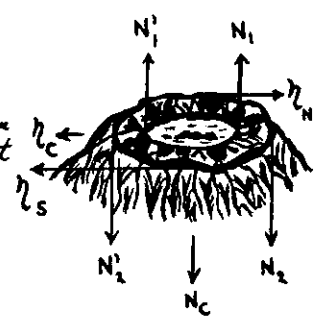
Depressions of larger and largest craters
