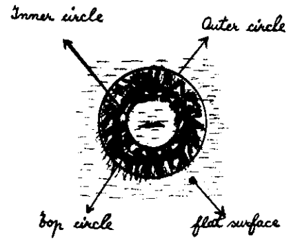
Non-extended rims crater.
